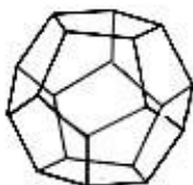
dodekahedron
